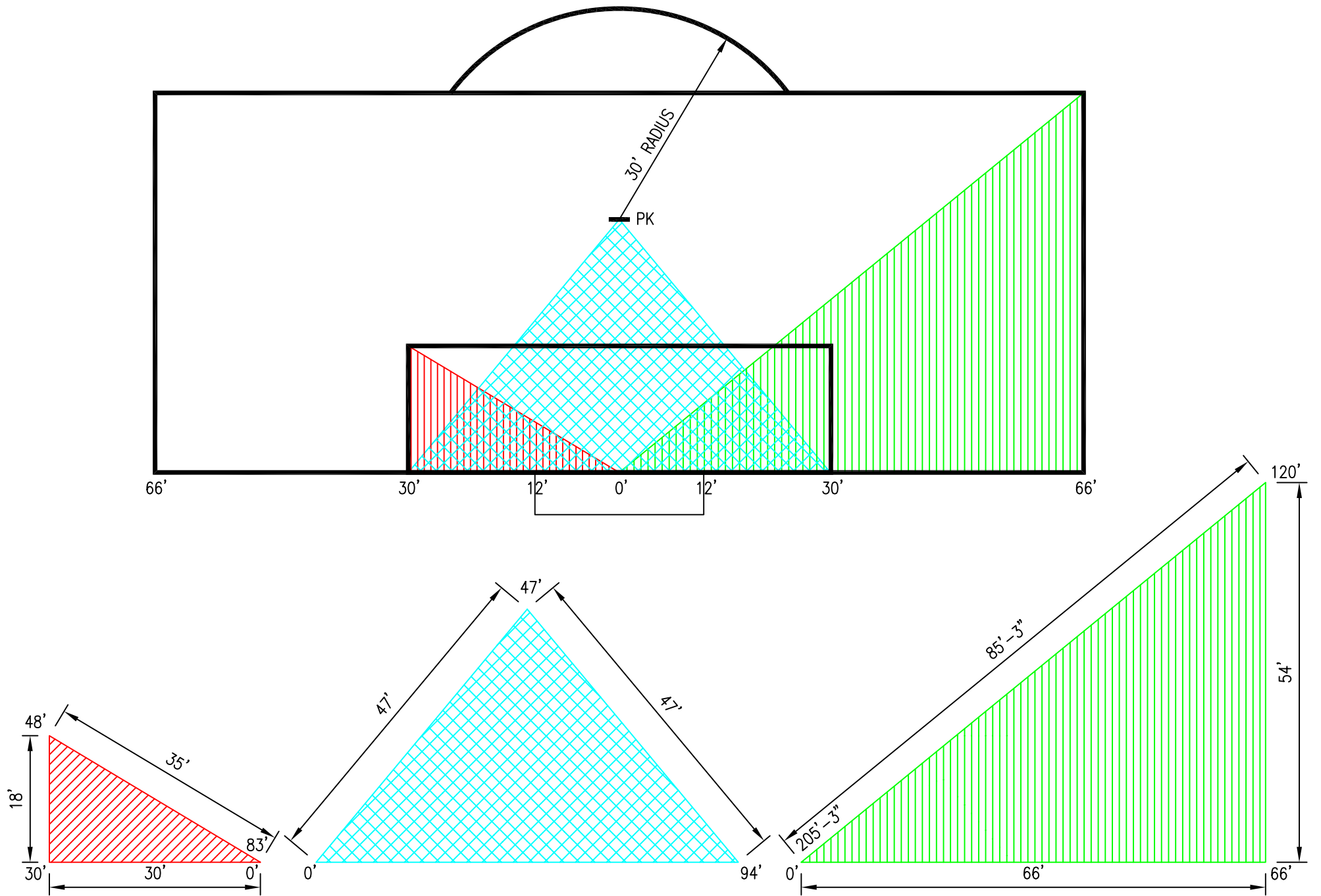
SOCCKER FIELD PENALTY AREA LAYOUT
